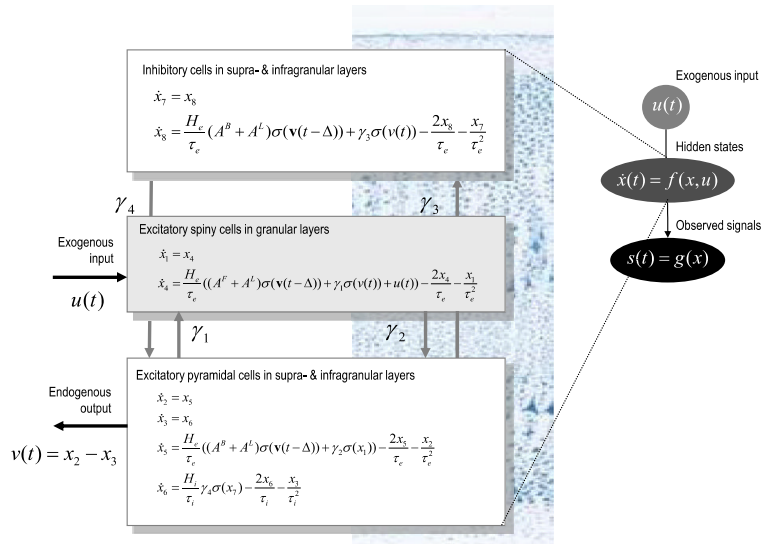
Fig. 2. Equations of motion for a single source. This schematic summarizes the equations of motion or state equations that specify a neural mass model of a single source. This model contains three sub-populations, each loosely associated with a specific cortical layer; corresponding roughly to spiny stellate input cells, deep pyramidal output cells and inhibitory interneurons. Following Felleman and Van Essen (1991), we distinguish between forward connections (targeting spiny stellate cells in the granular layer), backward connections (with slower kinetics and targeting pyramidal cells and inhibitory interneurons in both supra- and infragranular layers) and lateral connections (targeting all subpopulations). The output of each source is modeled as a parameterized mixture of the depolarization of each subpopulation (primarily the pyramidal cells). These delay differential equations describe changes in (vectors of) hidden states \mathbf{x}(t) (e.g., voltage and current) that subtend observed local field potentials or EEG signals. These delay differential equations effectively mediate a linear convolution of presynaptic activity to produce postsynaptic depolarization \mathbf{v}(t) . Average firing rates within each sub-population are then transformed through a nonlinear (sigmoid) voltage-firing rate function \sigma(\cdot) to provide inputs to other populations. These inputs are weighted by connection strengths. Here, \mathbf{v}(t - \Delta) represents a vector of (primarily) pyramidal depolarization in all sources, delayed by a connection-specific time-lag. Intrinsic connection strengths \gamma_i ; i = 1, \dots, 4 are shown connecting the different populations in different layers. When these equations are linearized around the system's fixed point, they specify the systems transfer function, and implicitly, the complex cross-spectra mapping from exogenous neuronal fluctuation or innovations \mathbf{u}(t) to observed responses \mathbf{s}(t) . These functions depend on the parameters of the model that include the extrinsic connection strengths and other parameters like H_j , \tau_j ; j \in \{i, e\} that control post-synaptic responses of inhibitory and excitatory populations. Under assumptions about the spectral form of the innovations, this constitutes a generative model of observed cross-spectra over multiple channels.
